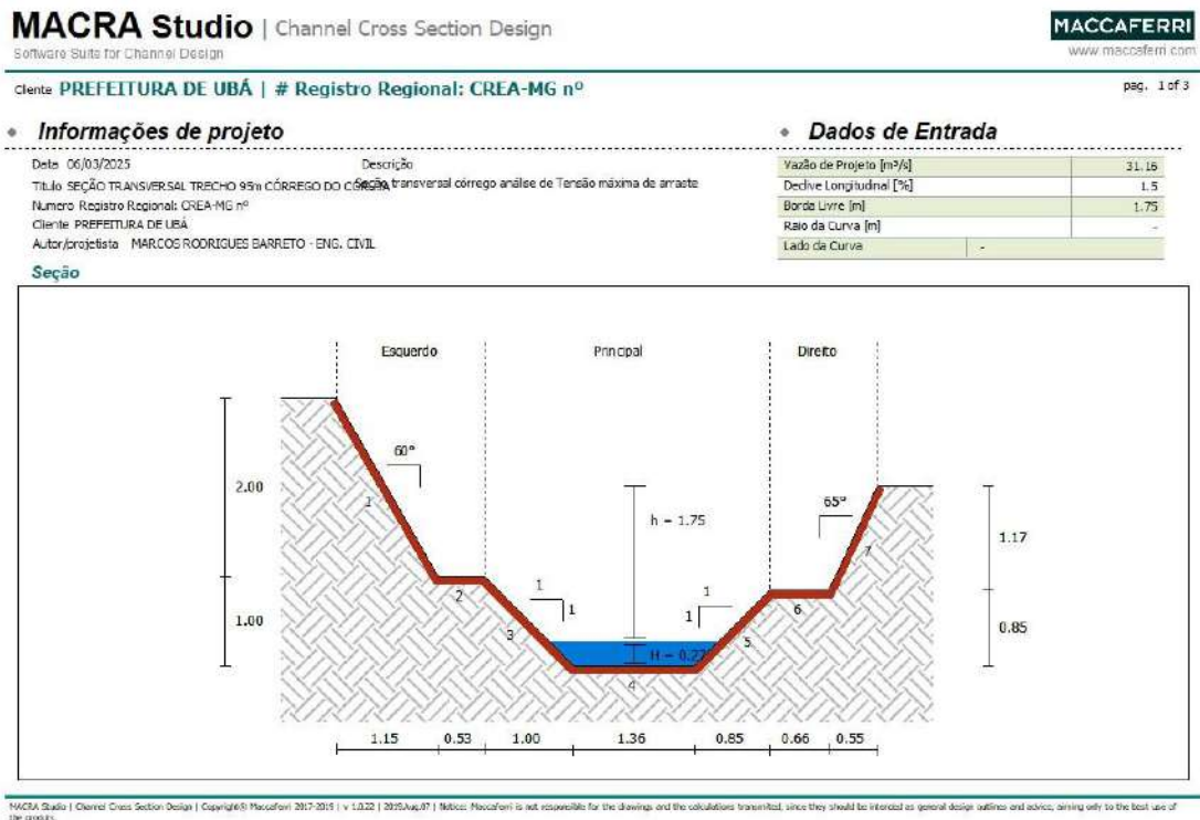
Figura 6 - MACRA Studio - Channel Cross Section Design (Seca)
