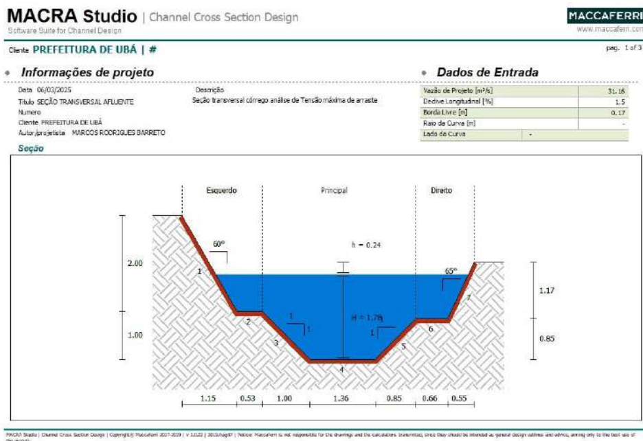
Figura 5 - MACRA Studio - Channel Cross Section Design (Cheia)
