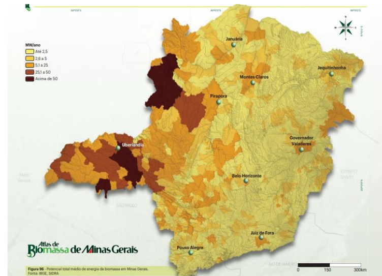
Potencial Biomassa
